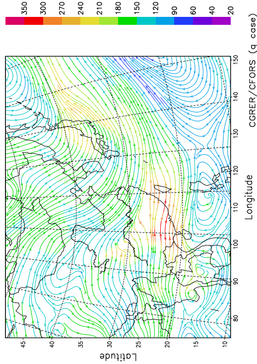
TRACE-P 31 MAR 2001 6 GMT Winds with Carbon Monoxide (ppb) at 3500 (m)
